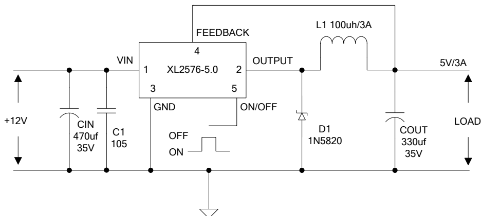
Figure4. XL2576 Typical Application Circuit 12V-5V/3A
