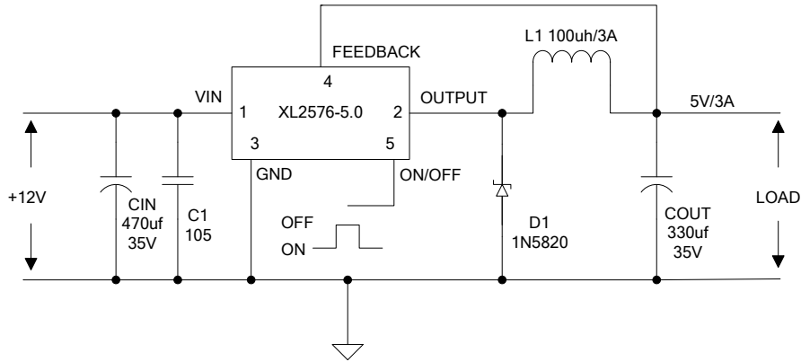
Figure6. XL2576-5.0 System Parameters Test Circuit
