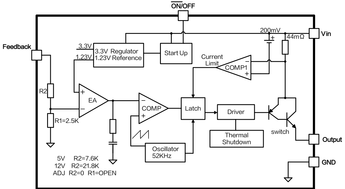
Figure3. Function Block Diagram of XL2576
