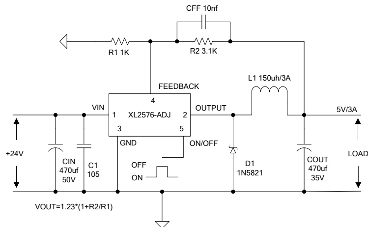
Figure8. XL2576-ADJ System Parameters Test Circuit
