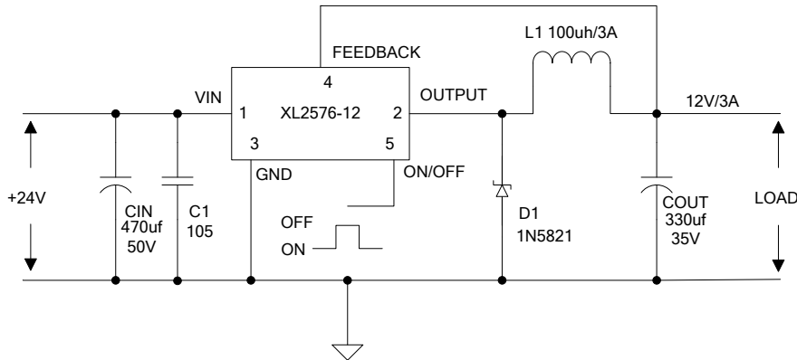
Figure7. XL2576-12 System Parameters Test Circuit
