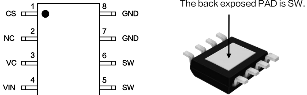
Figure2. Pin Configuration of XL3001
