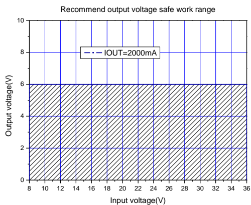
Figure9.Max output voltage(IOUT=2000mA)
