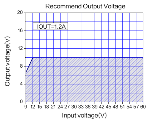
Figure21.Max Output Voltage ( I_{OUT}=1.2A , T_A=25^\circ C )
