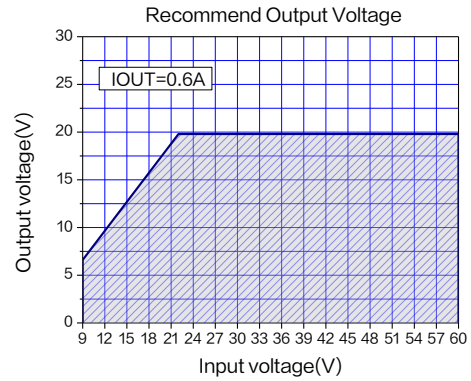
Figure19.Max Output Voltage ( I_{OUT}=0.6A , T_A=25^\circ C )
