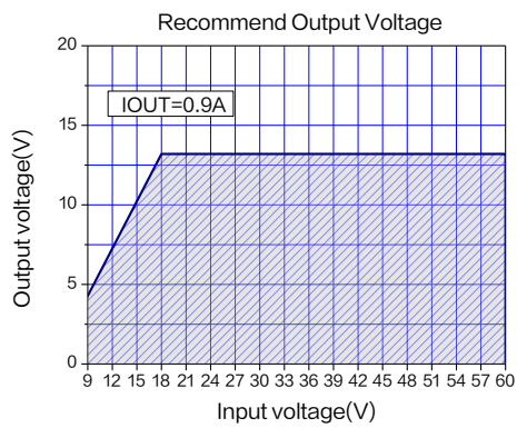
Figure20.Max Output Voltage ( I_{OUT}=0.9A , T_A=25^\circ C )
