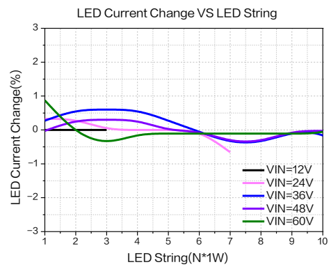
Figure15.Load Regulation
