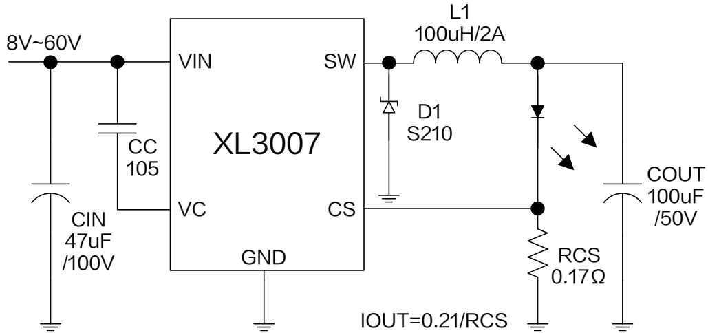
Figure10. XL3007 System Parameters Test Circuit ( V_{IN}=8V\sim60V, I_{OUT}=1.2A )
