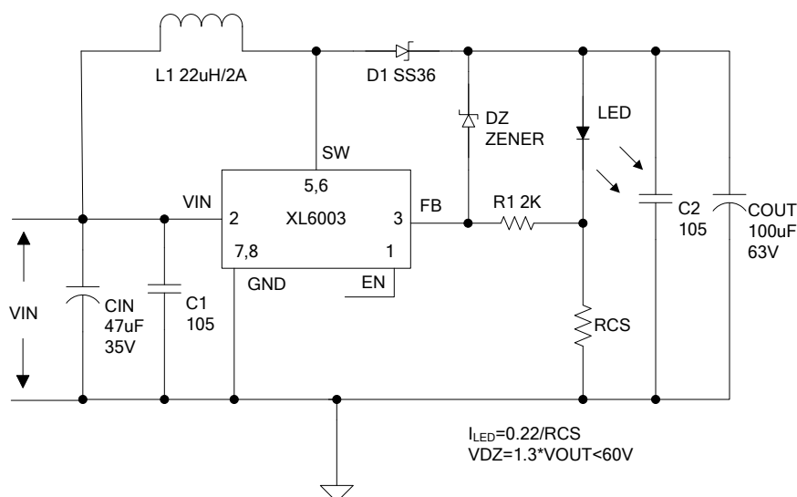
Figure10. XL6003 System Parameters Test Circuit (LED Open Protection)
