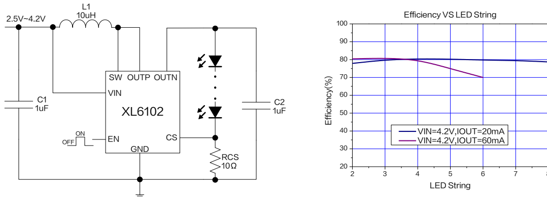
Figure4. XL6102 System Application and efficiency curve
