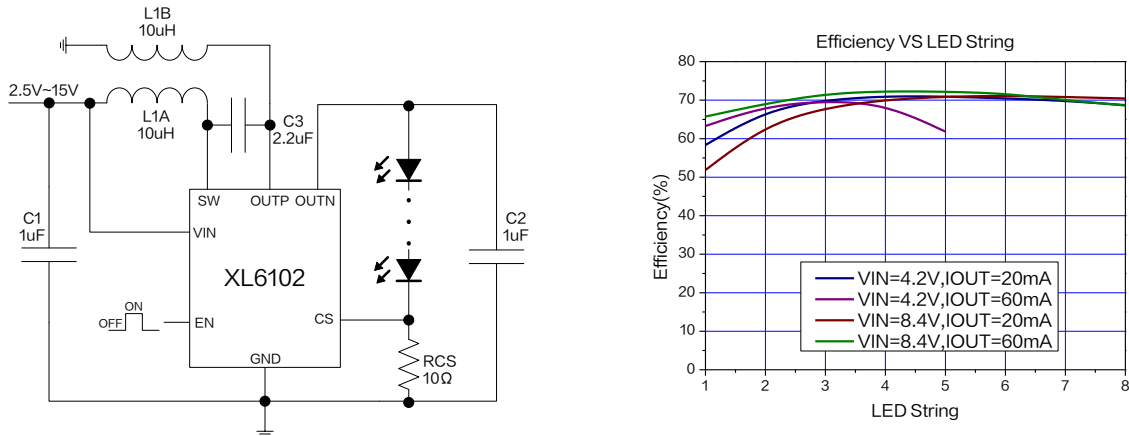
Figure7. XL6102 System Application and efficiency curve
