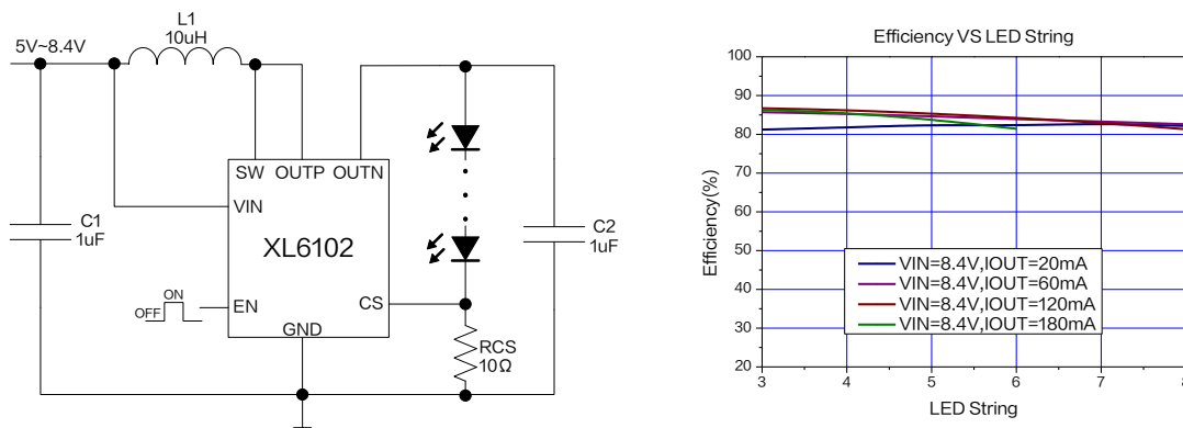
Figure5. XL6102 System Application and efficiency curve
