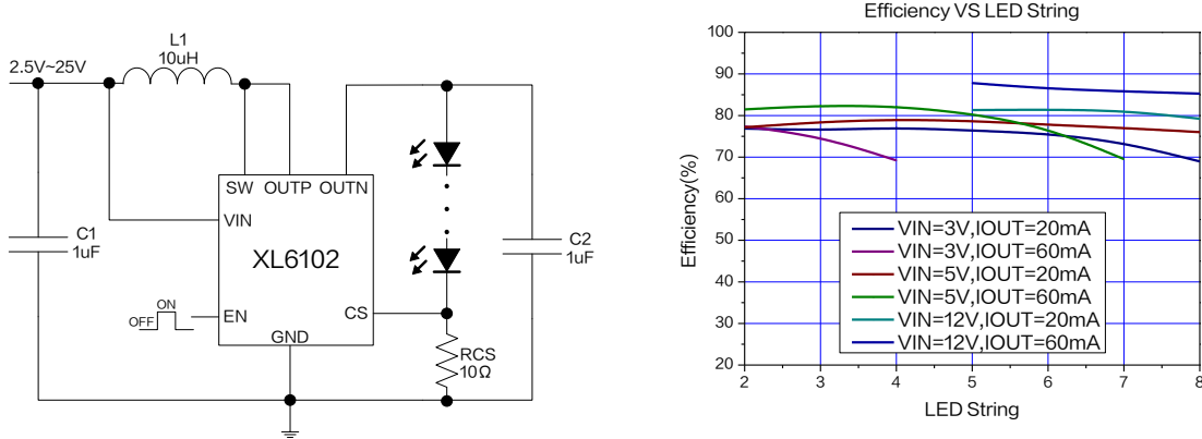
Figure6. XL6102 System Application and efficiency curve
