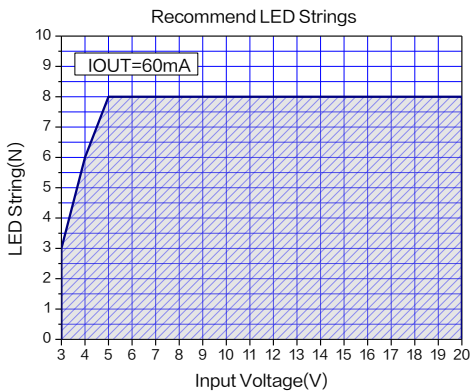
Figure 15.Max LED Strings( I_{OUT}=60mA )
