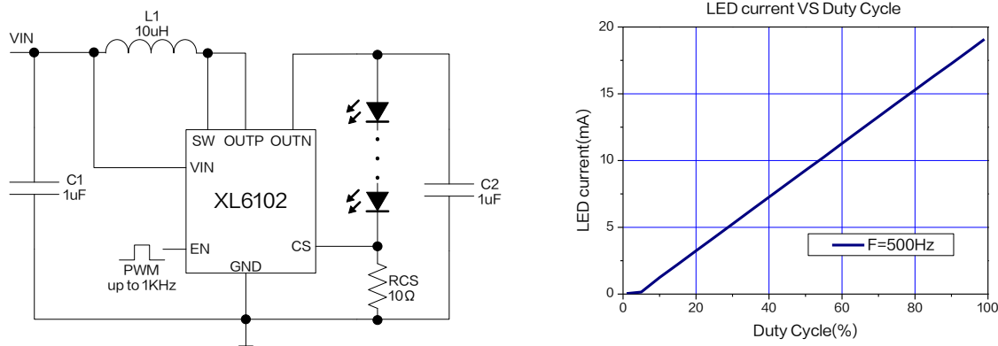
Figure 8. XL6102 Dimming circuit and PWM dimming curve
