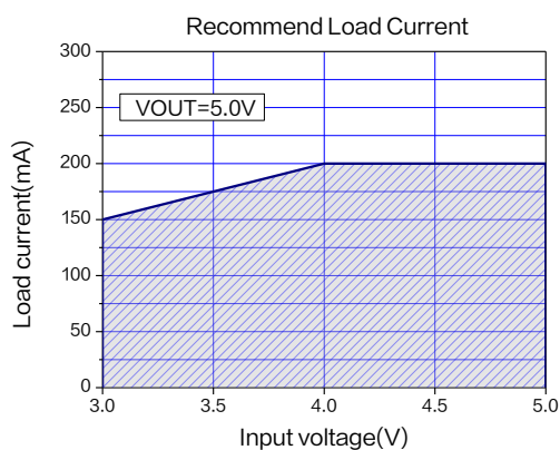
Figure 10. Max Output Current (V OUT =5.0V, T A =25°C)
