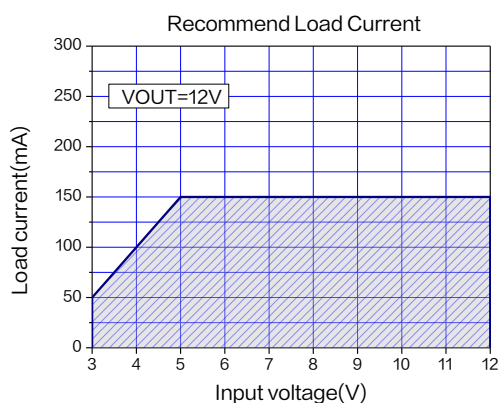
Figure 12. Max Output Current (V OUT =12V, T A =25°C)
