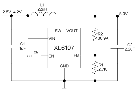
Figure4. XL6107 System Application and efficiency curve ( V_{OUT}=5.0V )
