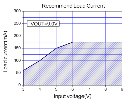
Figure 11. Max Output Current (V OUT =9.0V, T A =25°C)
