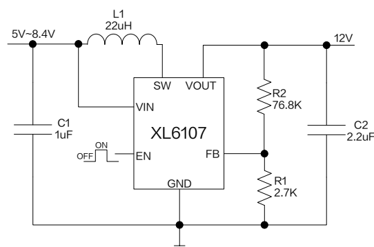
Figure5. XL6107 System Application and efficiency curve ( V_{OUT}=12V )
