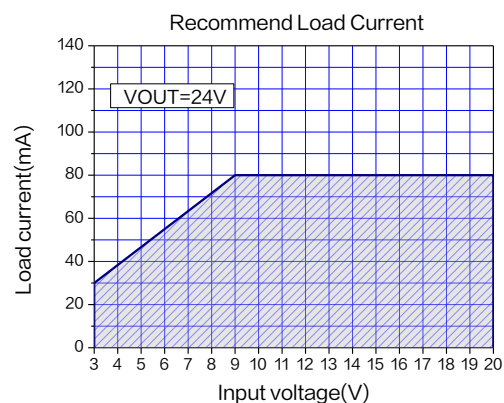
Figure 13. Max Output Current (V OUT =24V, T A =25°C)
