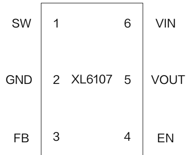
Figure2. Pin Configuration of XL6107
