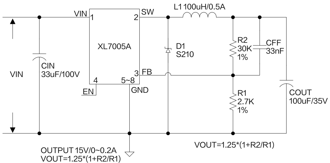
Figure4. XL7005A Typical Application Circuit
