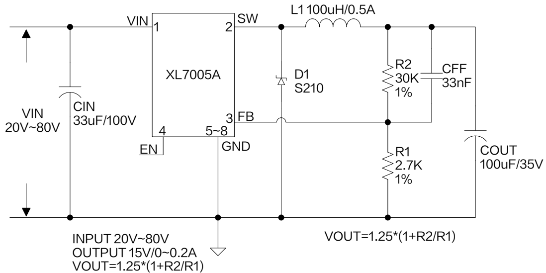
Figure8. XL7005A System Application (V IN =20V~80V, V OUT =15V/0.2A)
