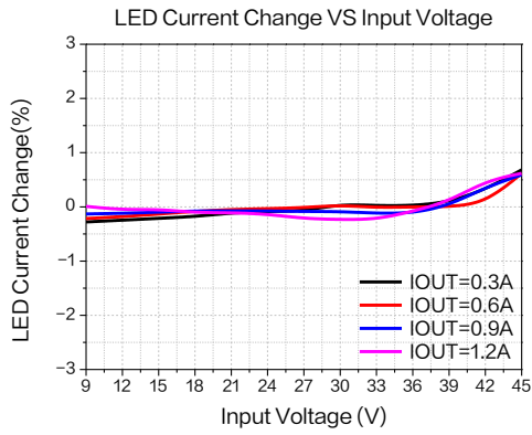
Figure14.Line Regulation
