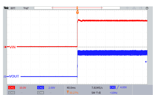
Figure25. Start-Up Characteristic ( V_{IN}=36V , V_{OUT}=6.6V , I_{OUT}=0.3A )
