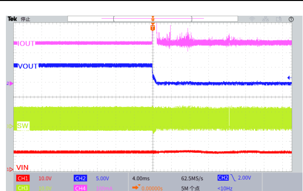
Figure27. LED Short Protection ( V_{IN}=12V , V_{OUT}=6.6V , I_{OUT}=0.3A )
