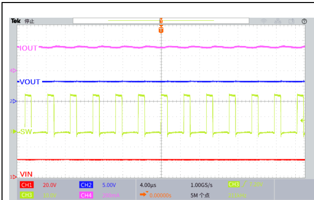
Figure29. LED Current Ripple ( V_{IN}=24V , V_{OUT}=9.9V , I_{OUT}=0.3A )
