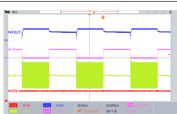
Figure32. Start or Shutdown Using EN Pin ( V_{IN}=12V , V_{OUT}=6.6V , I_{OUT}=0.3A )
