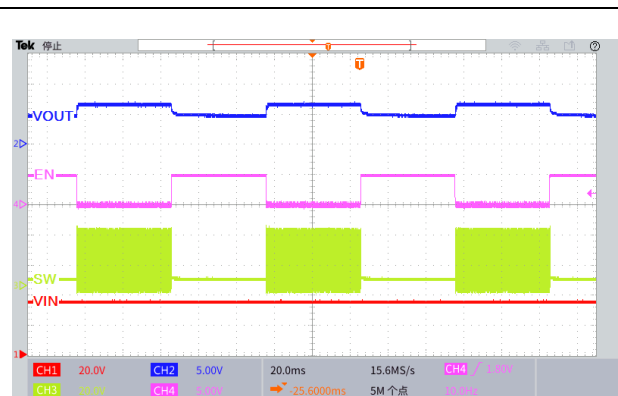
Figure34. Start or Shutdown Using EN Pin ( V_{IN}=36V , V_{OUT}=6.6V , I_{OUT}=0.3A )
