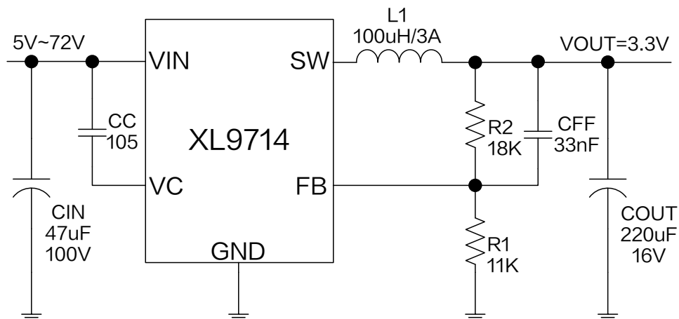
Figure4. XL9714 System Application ( V_{IN}=5V\sim72V , V_{OUT}=3.3V , I_{OUT}=0\sim1.5A )
