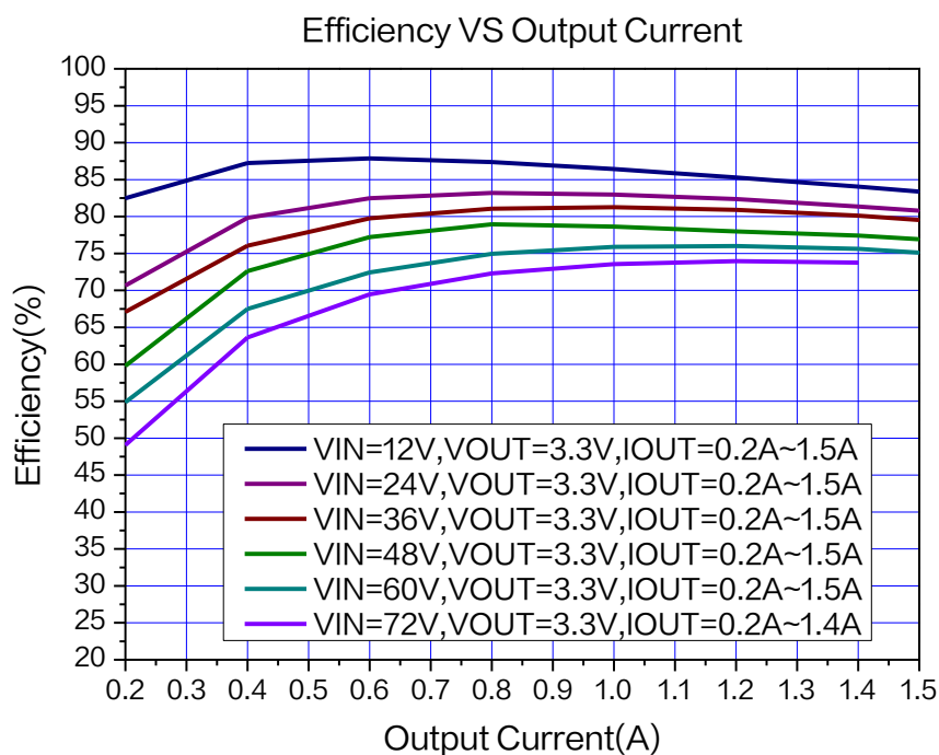
Figure5. XL9714 System Efficiency Curve( V_{OUT}=3.3V )
