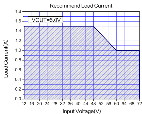
Figure 15.Max Output Current ( V_{OUT}=5.0V , T_A=25^{\circ}C )
