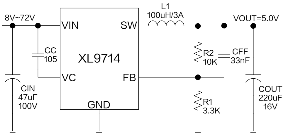
Figure6. XL9714 System Application ( V_{IN}=8V\sim72V , V_{OUT}=5.0V , I_{OUT}=0\sim1.5A )
