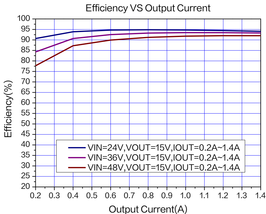
Figure9. XL9714 System Efficiency Curve ( V_{OUT}=15V )
