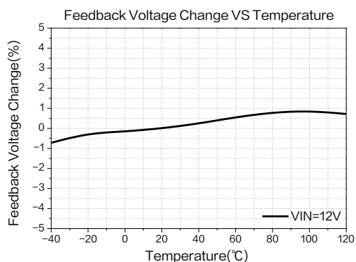
Figure 12.Feedback Voltage Regulation
