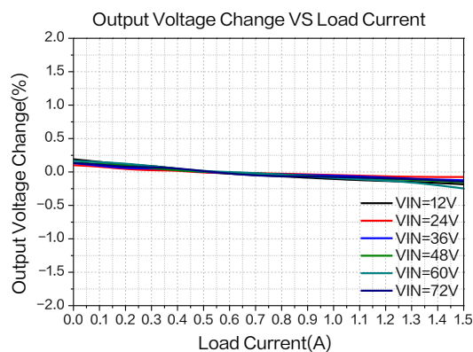
Figure 11.Load Regulation
