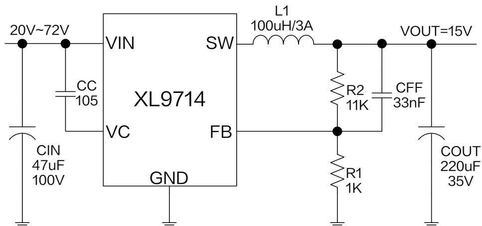
Figure8. XL9714 System Application ( V_{IN}=20V\sim72V , V_{OUT}=15V , I_{OUT}=0\sim1.4A )
