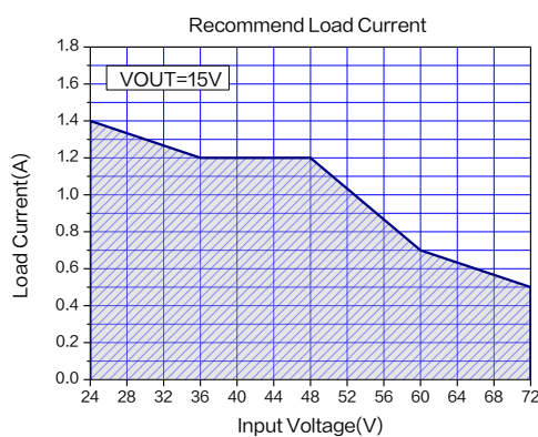
Figure 17.Max Output Current ( V_{OUT}=15V , T_A=25^{\circ}C )
