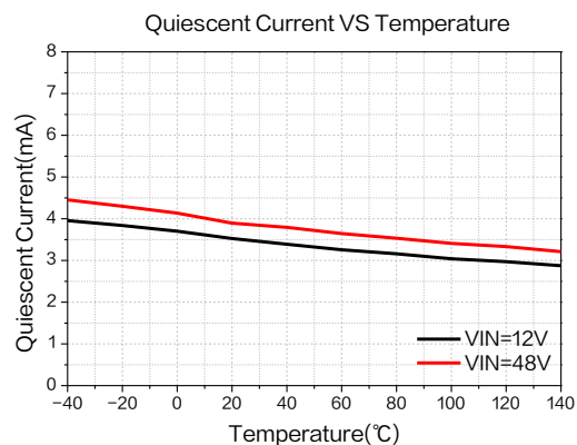
Figure 13.Quiescent Current
