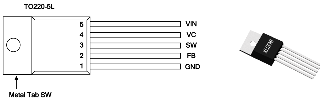
Figure2. Pin Configuration of XL9714
